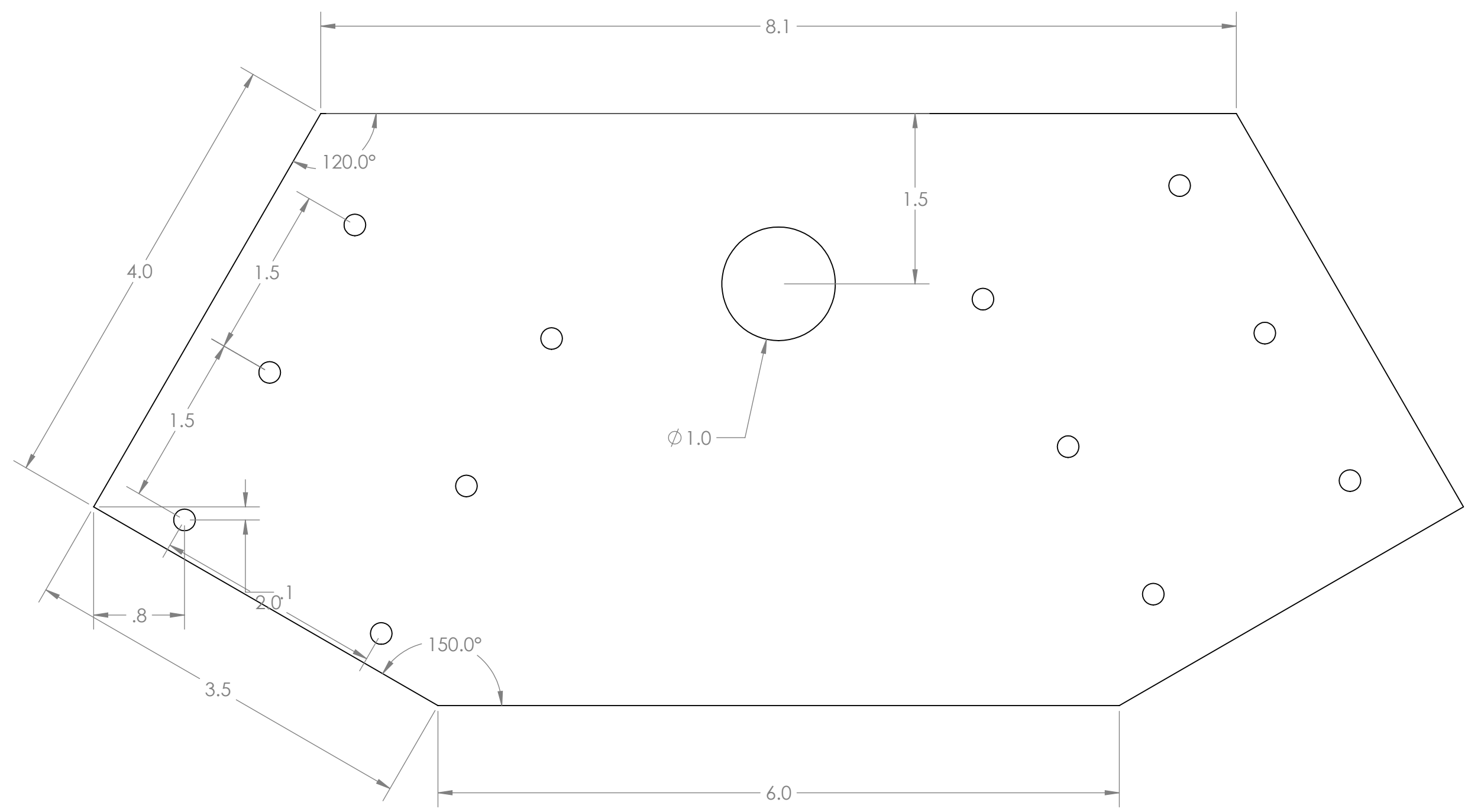
SUPPORT TOP PLATE (SUPPORT-4)
