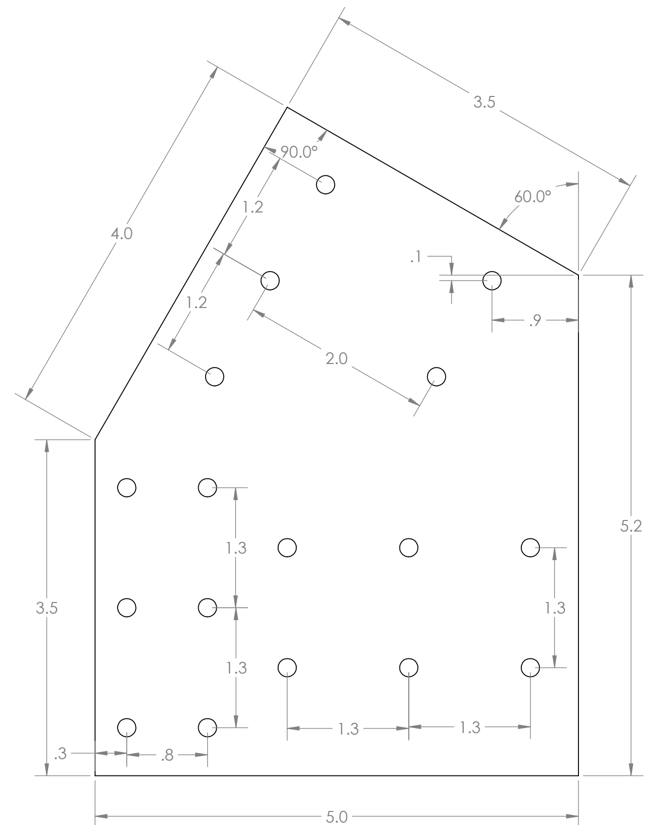
SUPPORT SIDE PLATE (SUPPORT-1)
