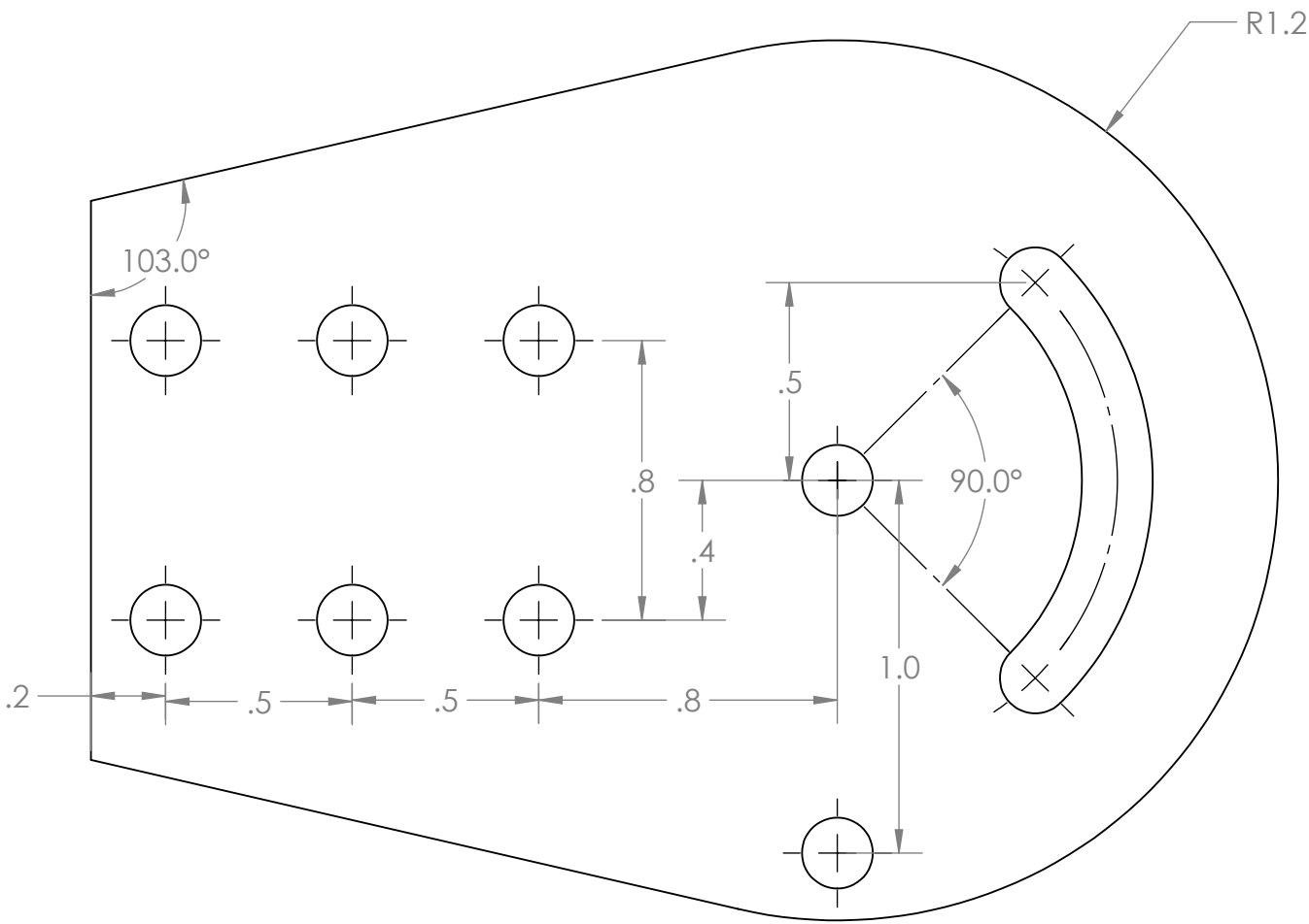
COUNTERWEIGHT ANGLE LIMIT PLATE (ARM-6)
