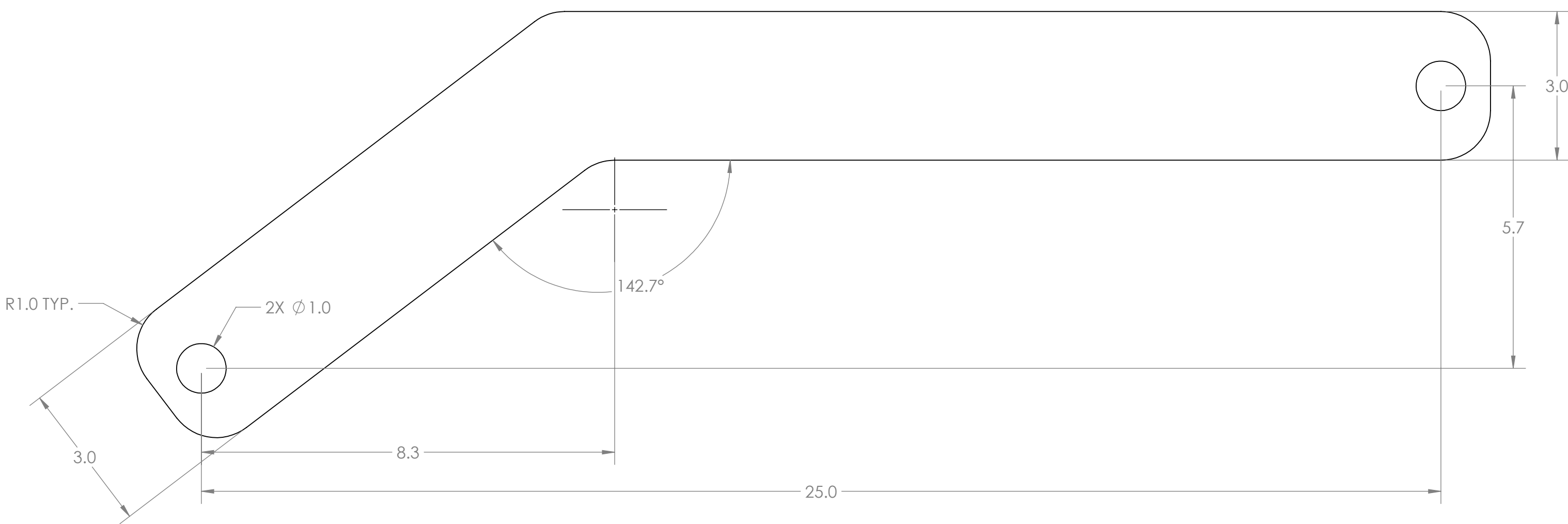
COUNTERWEIGHT ARM (COUNTERWEIGHT-1)
