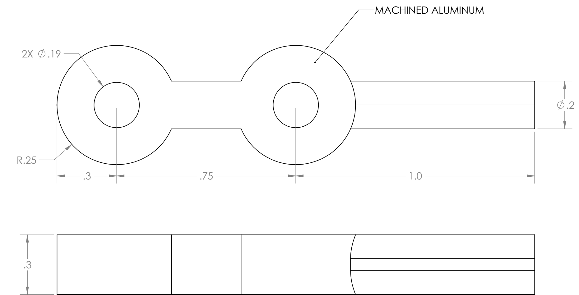
RELEASE PIN (PIN)
