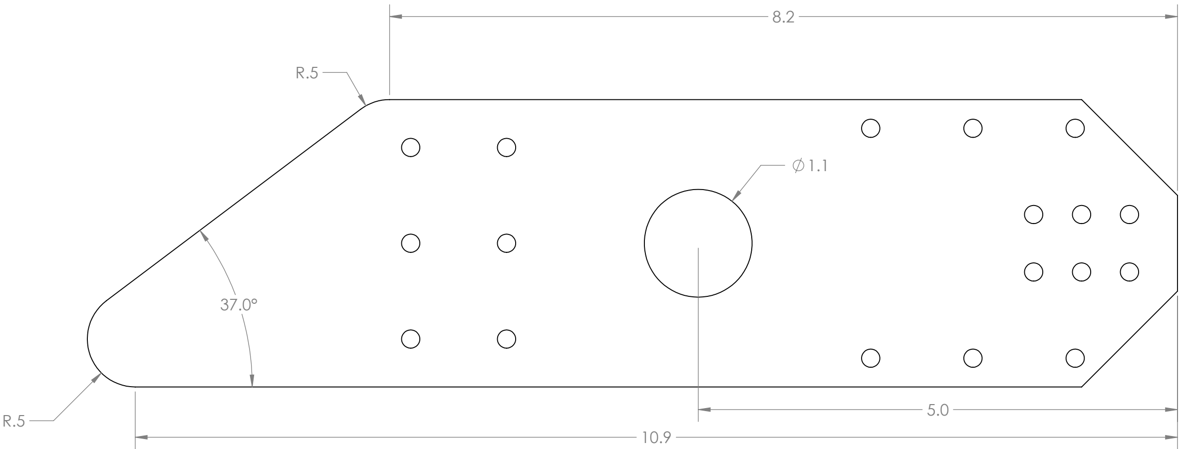
COUNTERWEIGHT ANGLE LIMIT PLATE (ARM-6)
