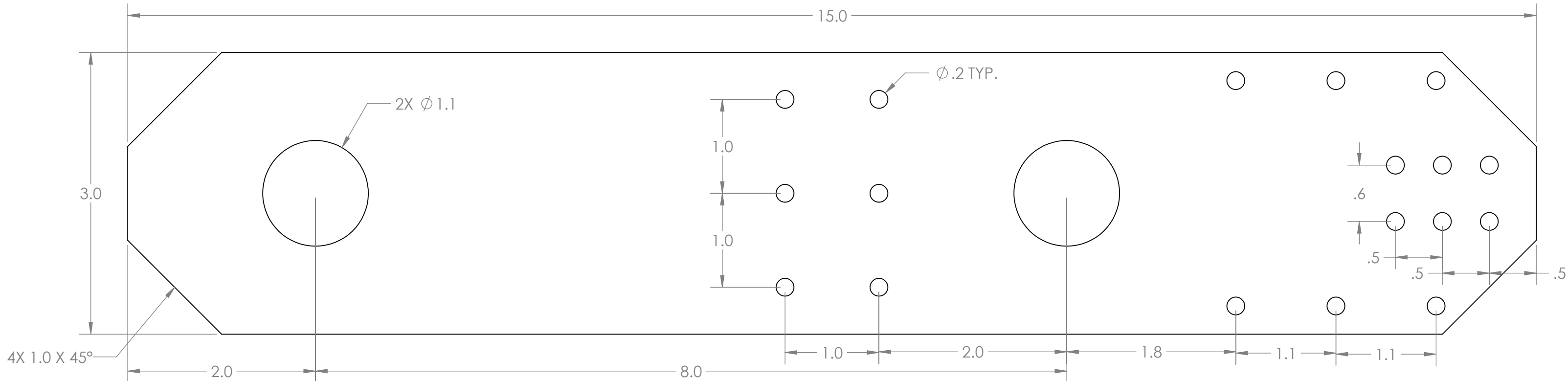
ARM PLATE 1 (ARM-2)
